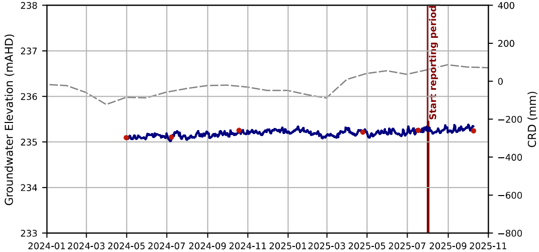
Hydrograph - WR1
