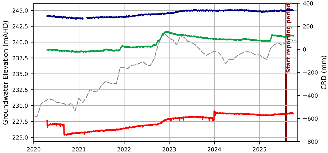
Hydrograph - VS059
