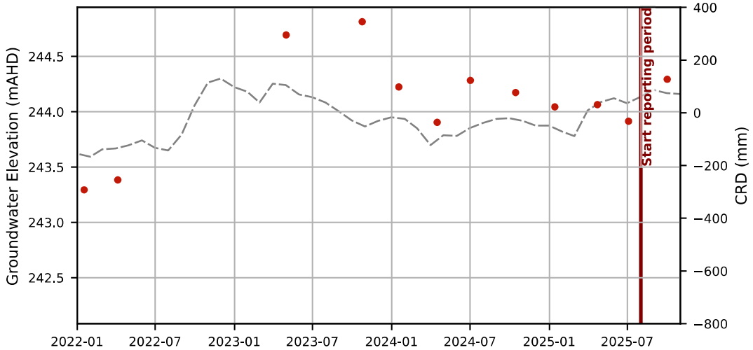
Hydrograph - SB11
