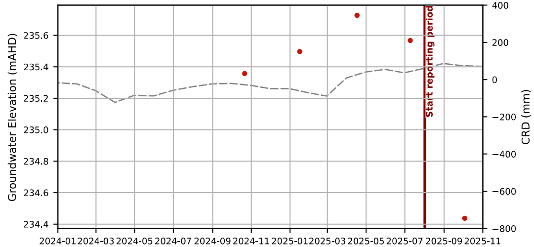
Hydrograph - GW-14
