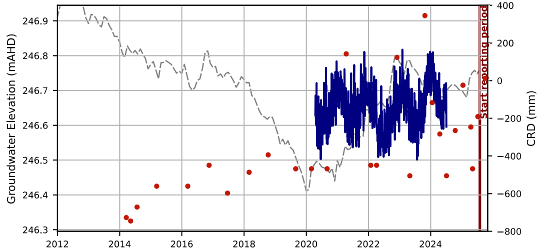
Hydrograph - TR18
