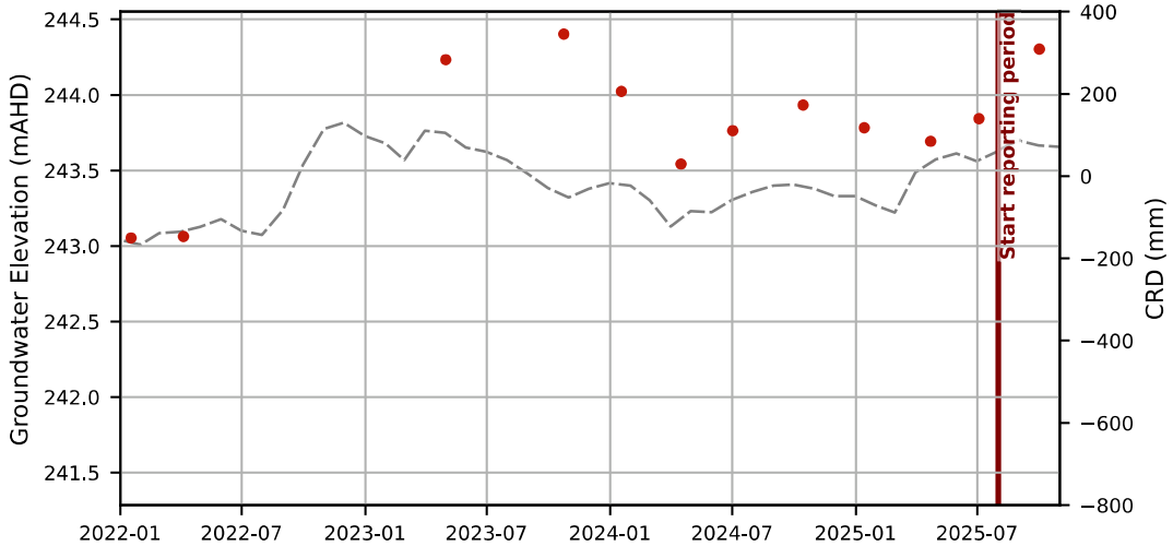
Hydrograph - SB05
