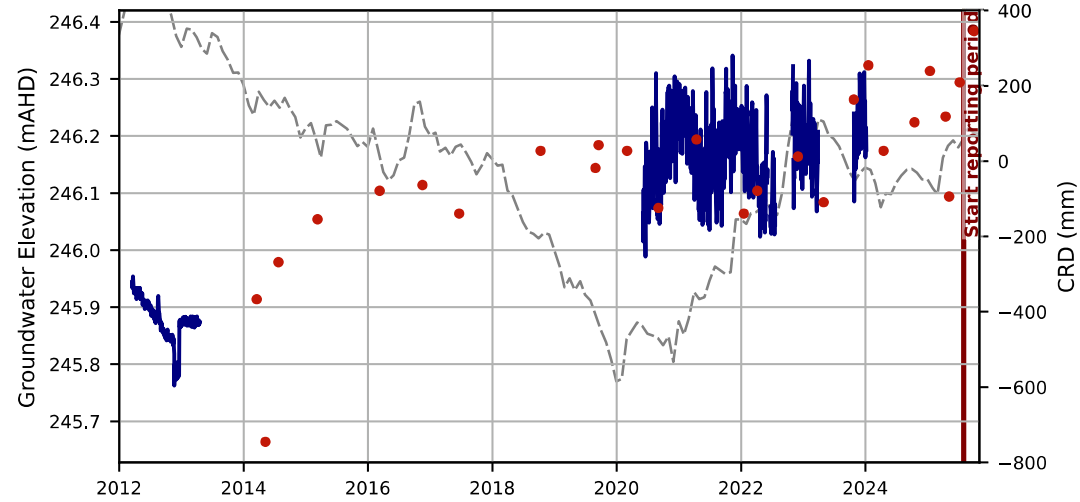
Hydrograph - TR7
