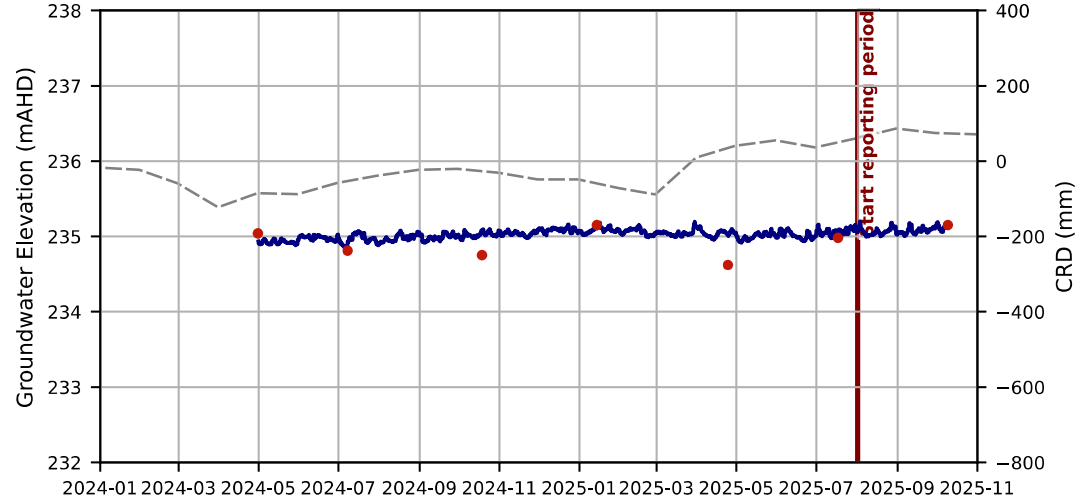
Hydrograph - WR2
