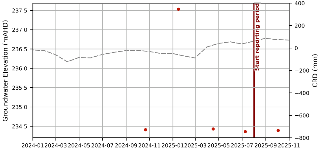
Hydrograph - GW-13
