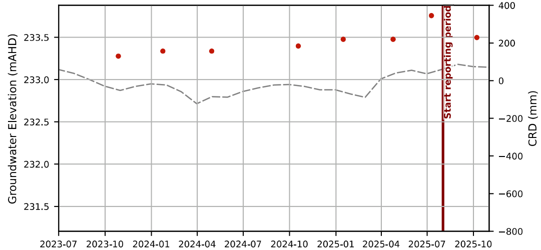
Hydrograph - GW-11
