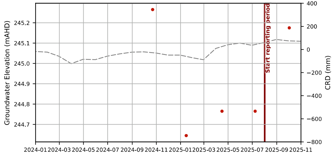
Hydrograph - GW-15
