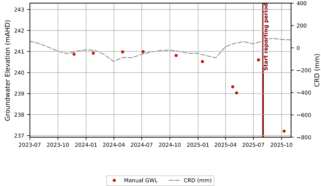
Hydrograph - GW-8
