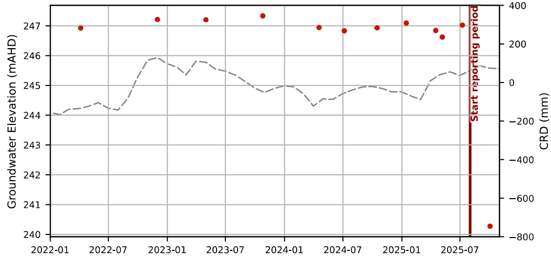
Hydrograph - TR35
