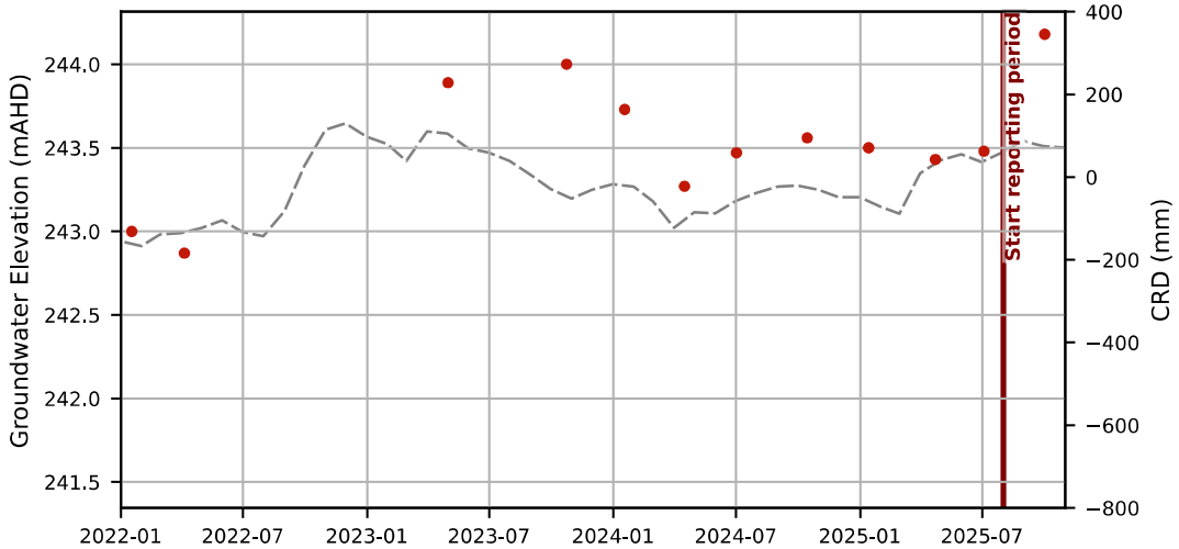
Hydrograph - SB09
