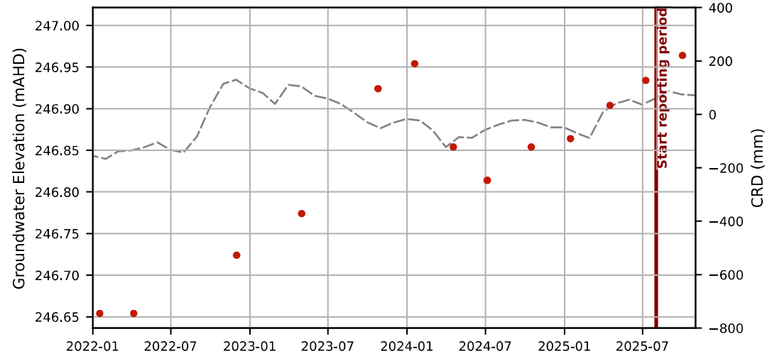
Hydrograph - TR26
