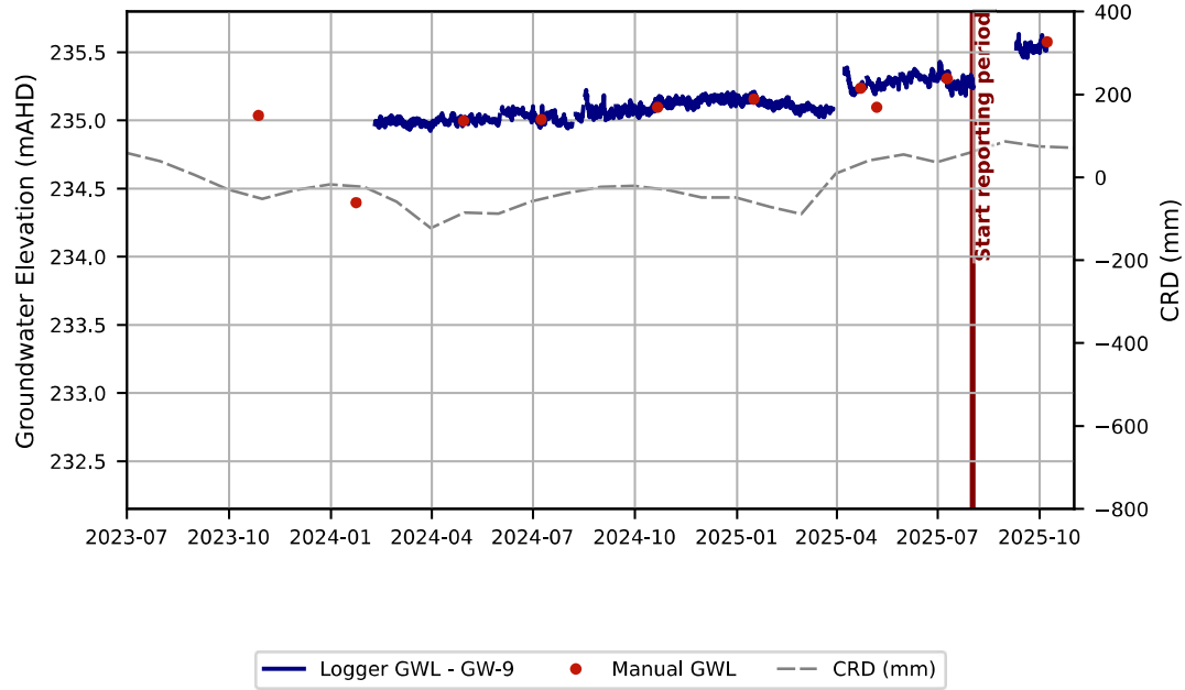
Hydrograph - GW-9
