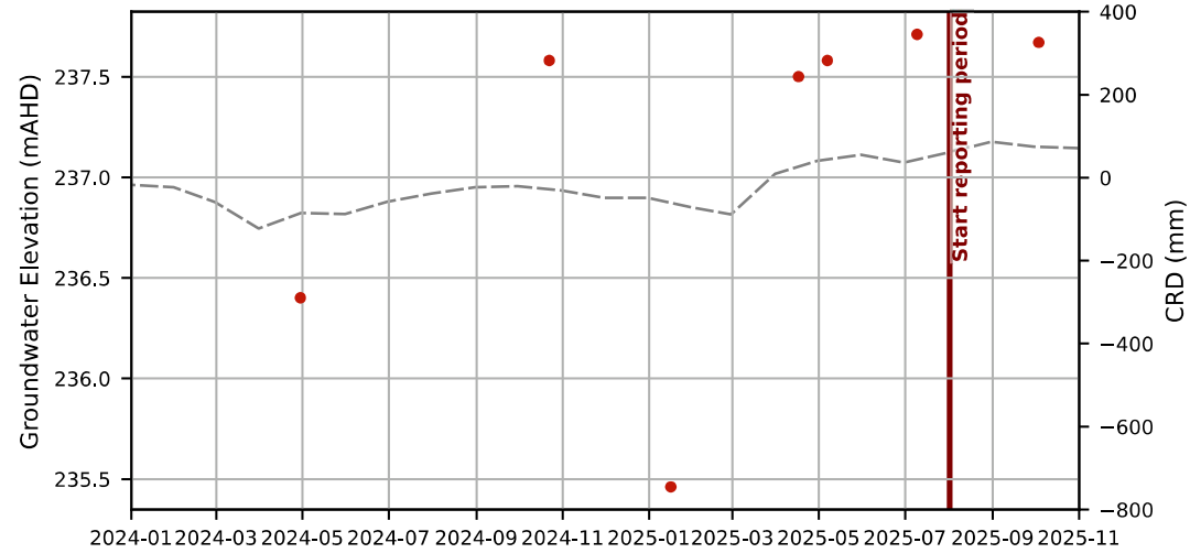
Hydrograph - GW-2
