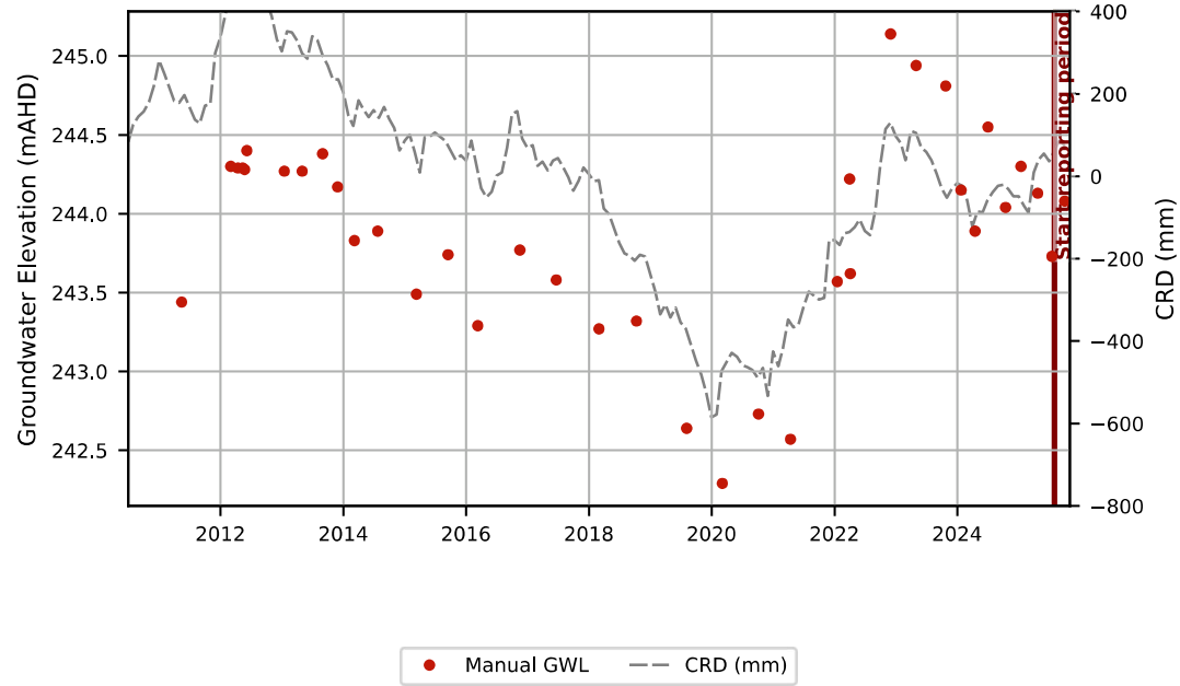
Hydrograph - GW01
