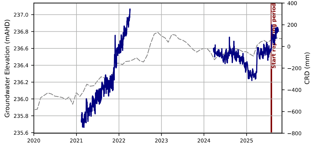
Hydrograph - VS062
