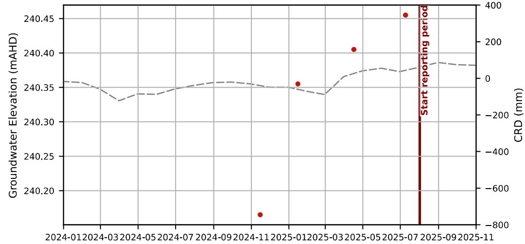
Hydrograph - GW-6
