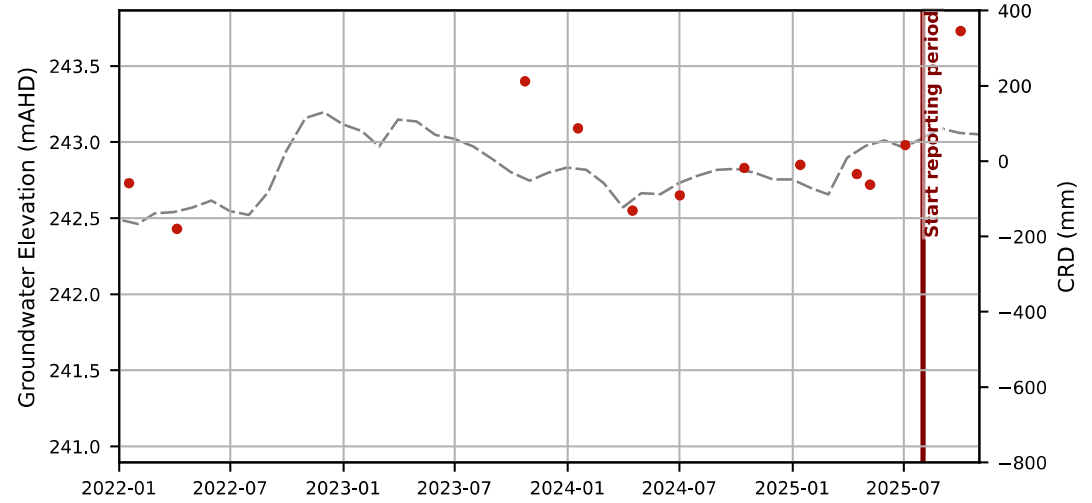
Hydrograph - SB04
