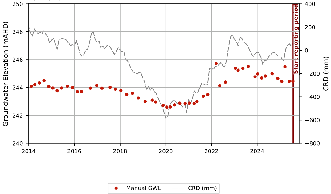
Hydrograph - GW036459
