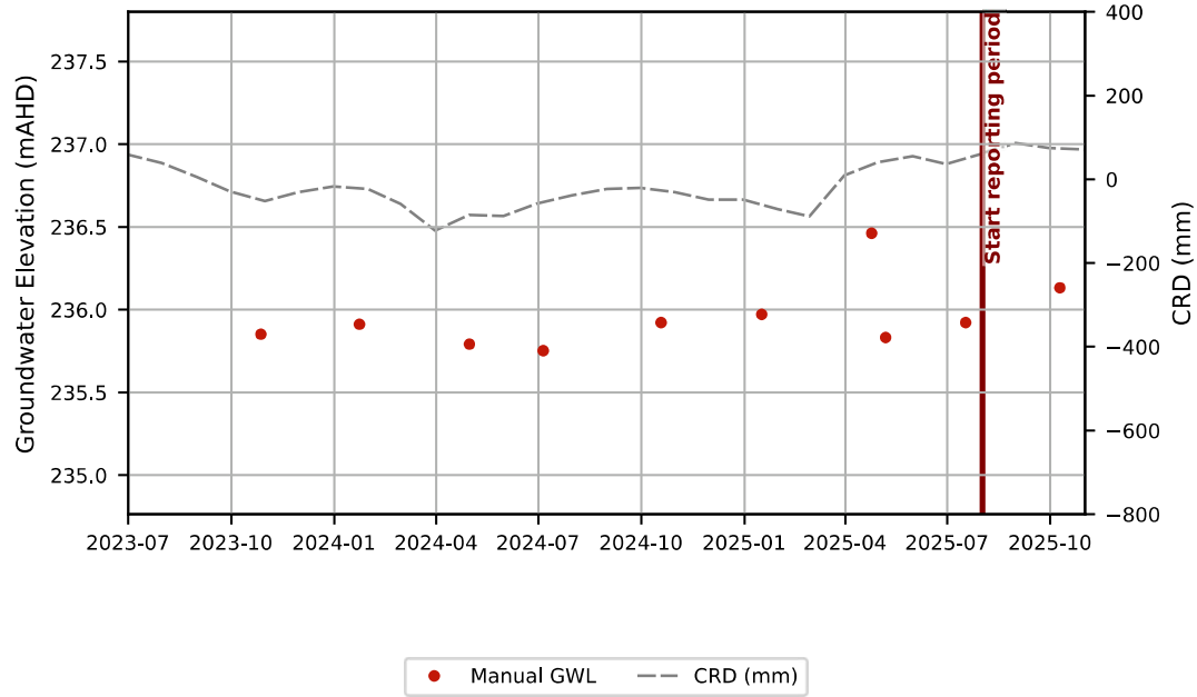
Hydrograph - GW-7
