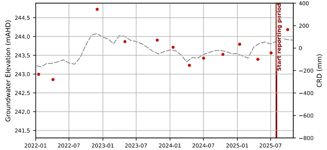
Hydrograph - SB01
