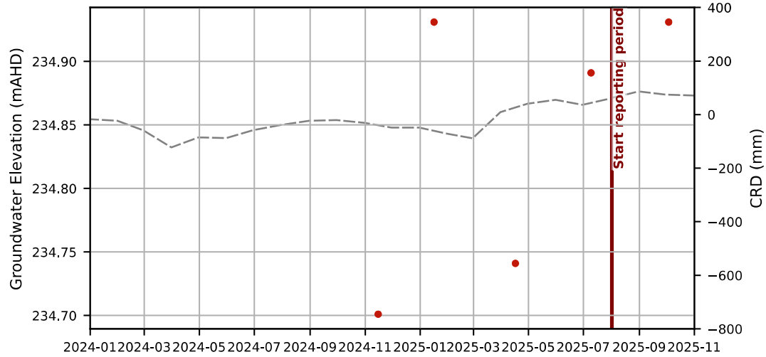
Hydrograph - GW-4
