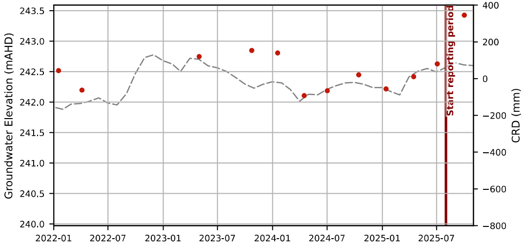
Hydrograph - SB07
