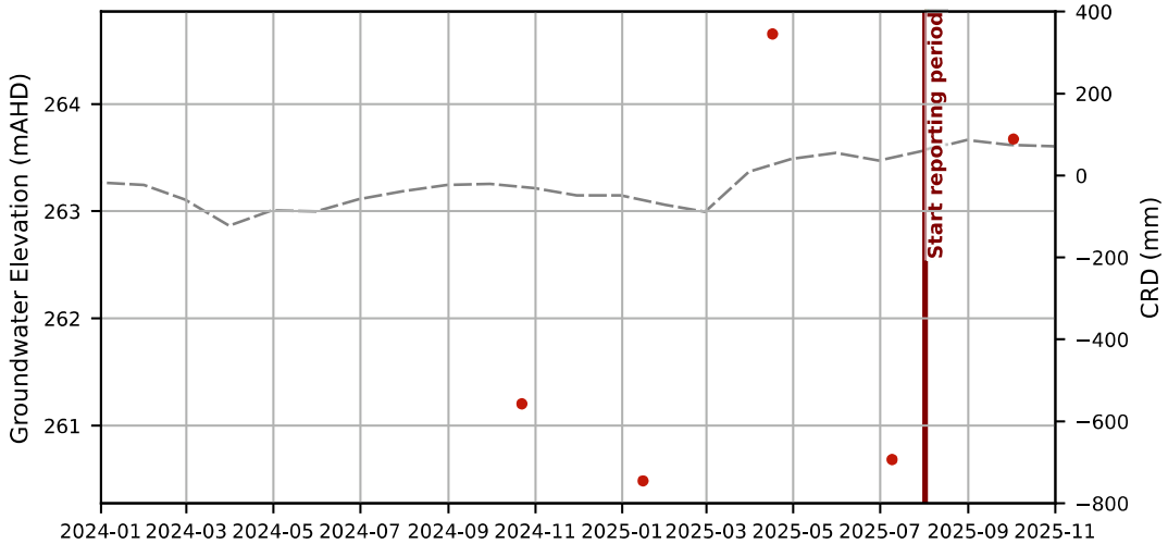
Hydrograph - GW-10
