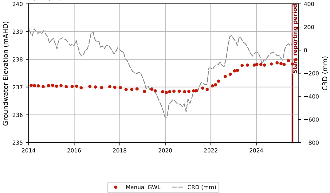
Hydrograph - GW030052-1
